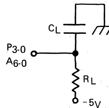
LOAD CIRCUIT
