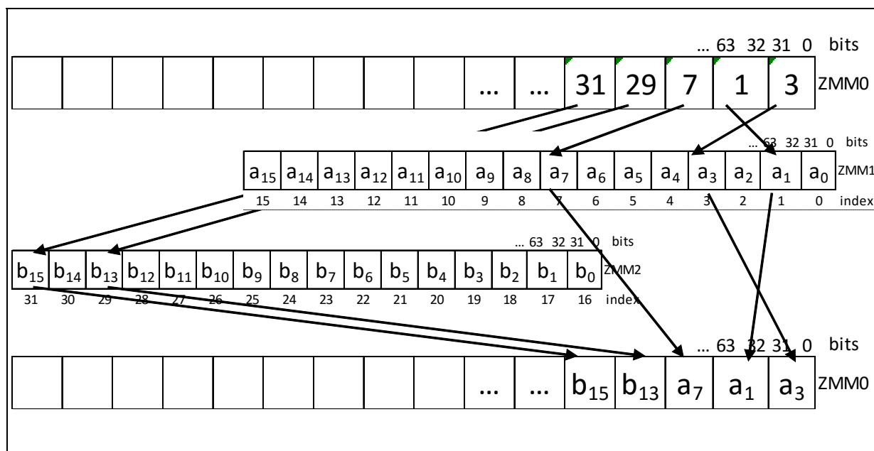
Figure 13-8. vpermi2ps Operation
