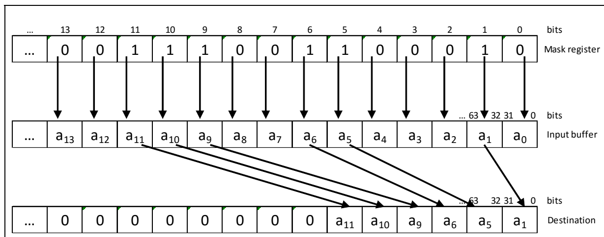
Figure 13-4. Data Compress Operation
