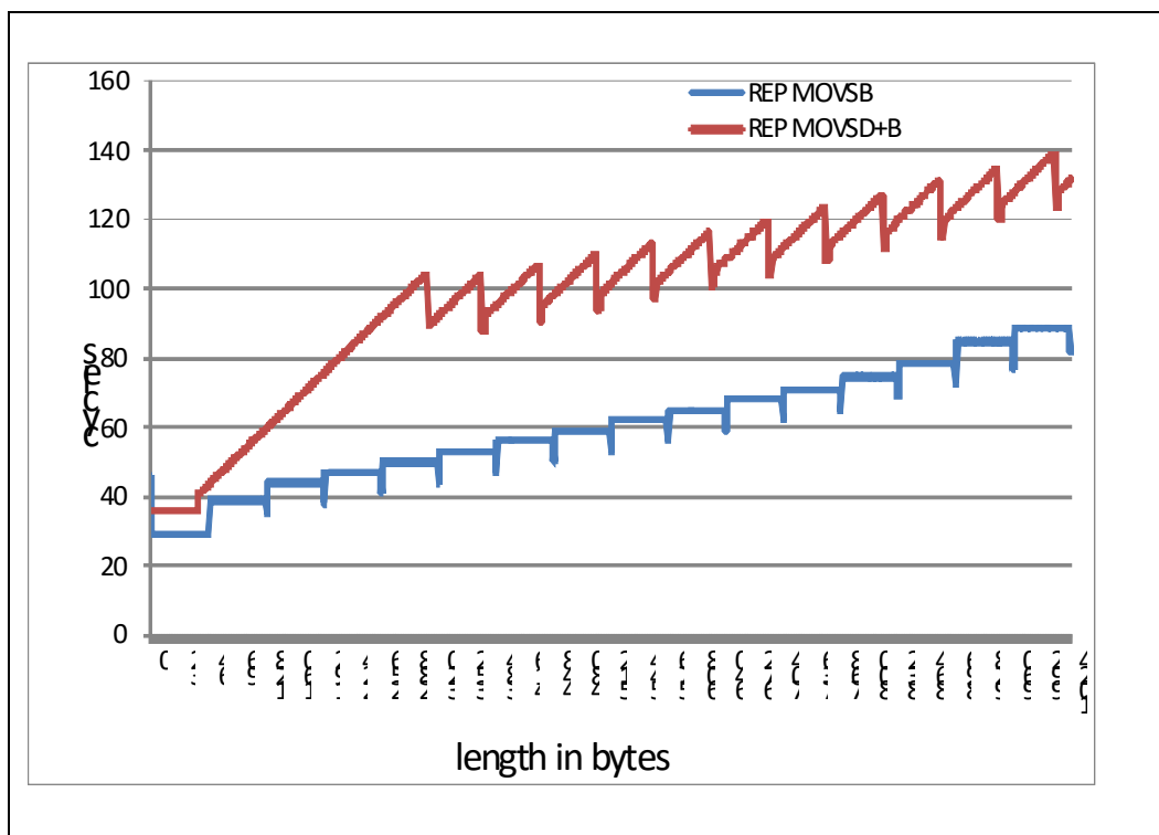
Figure 3-4. Malloc Performance Comparison for Lengths up to 2KB
