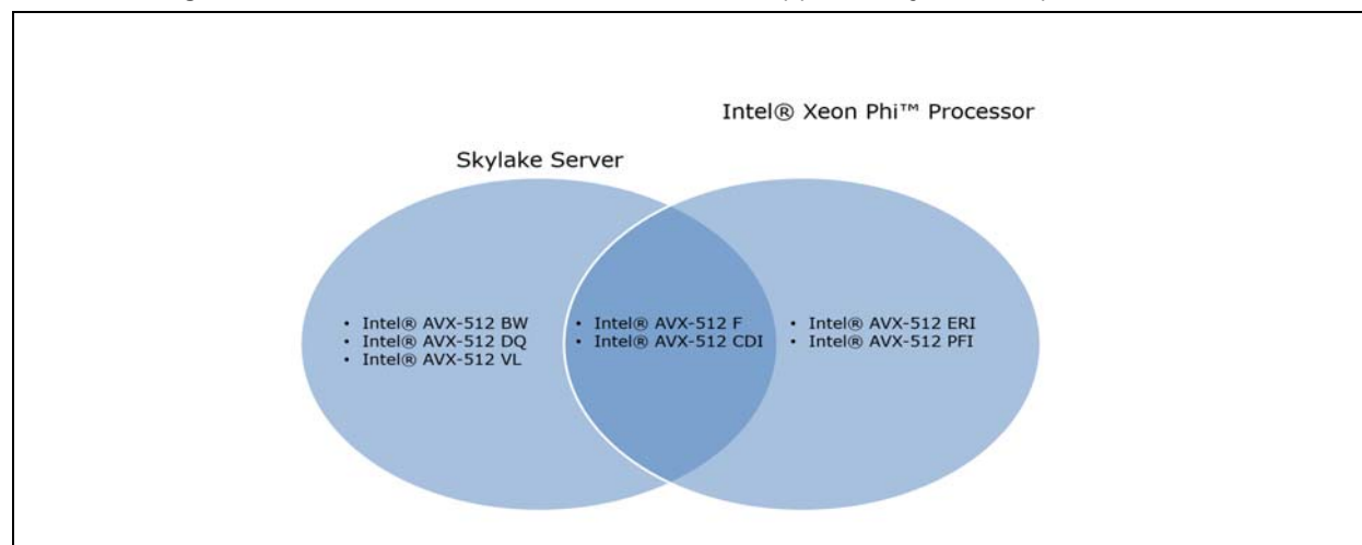
Figure 13-1. Intel® AVX-512 Extensions Supported by Skylake Server Microarchitecture and Knights Landing Microarchitecture
