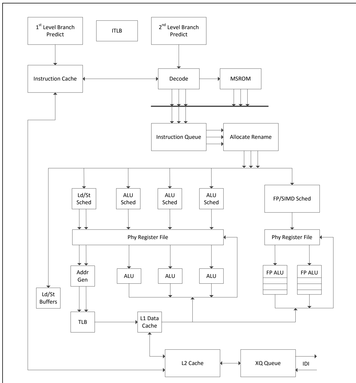
Figure 16-1. CPU Core Pipeline Functionality of the Goldmont Microarchitecture
