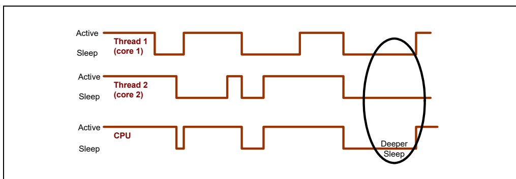
Figure 15-6. Progression to Deeper Sleep
