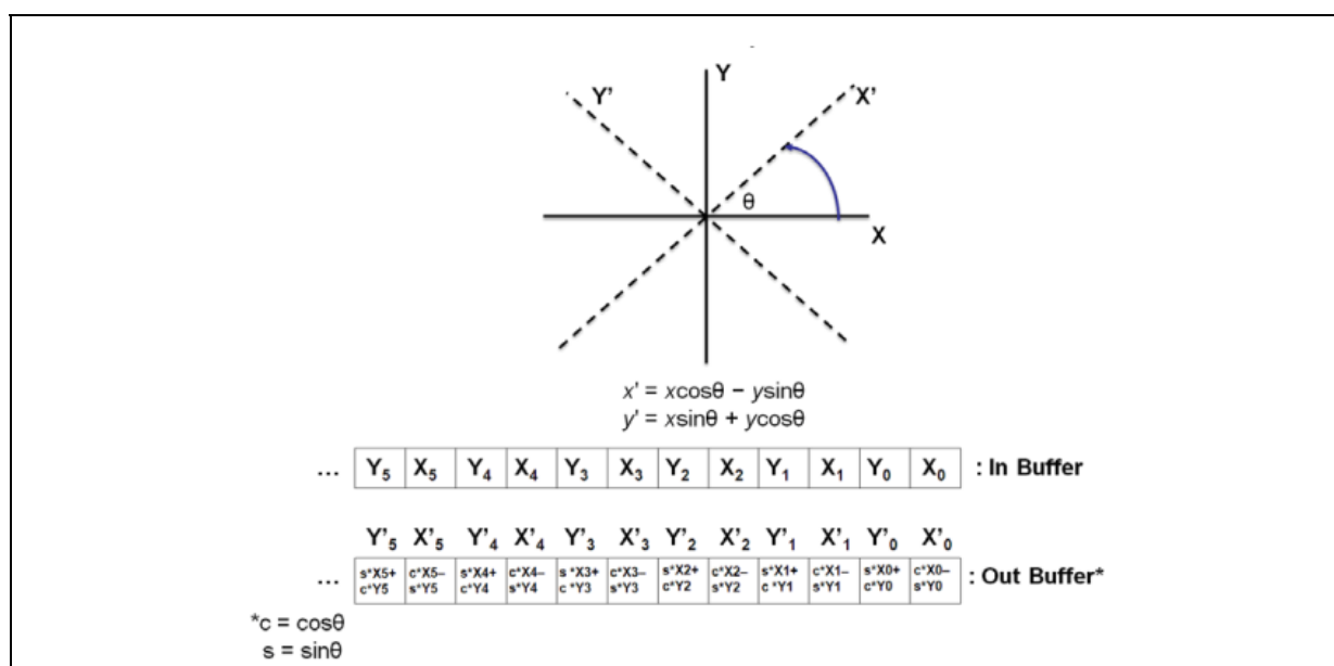
Figure 13-2. Cartesian Rotation
