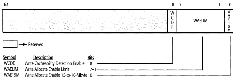
Figure 30. Write Handling Control Register (WHCR)—MSR C000_0082h
