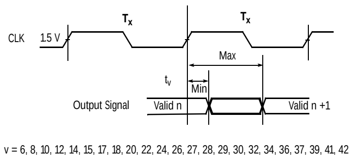
Figure 11. Output Valid Delay Timing
