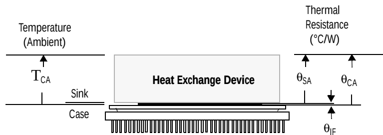
Figure 30. Thermal Model
