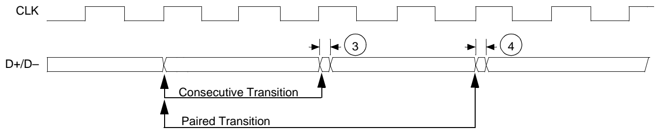
Figure 36. USB Receiver Jitter Tolerance
