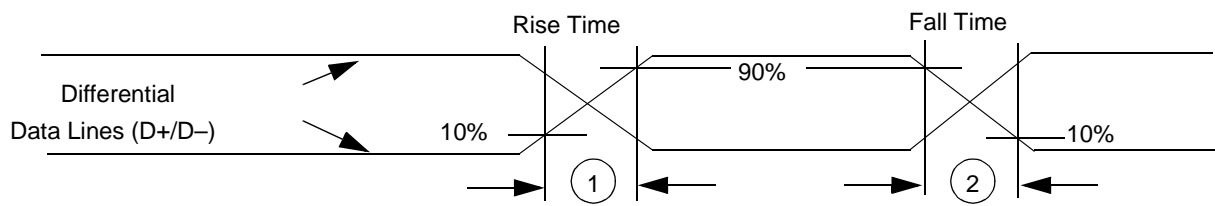
Figure 35. USB Data Signal Rise and Fall Times
