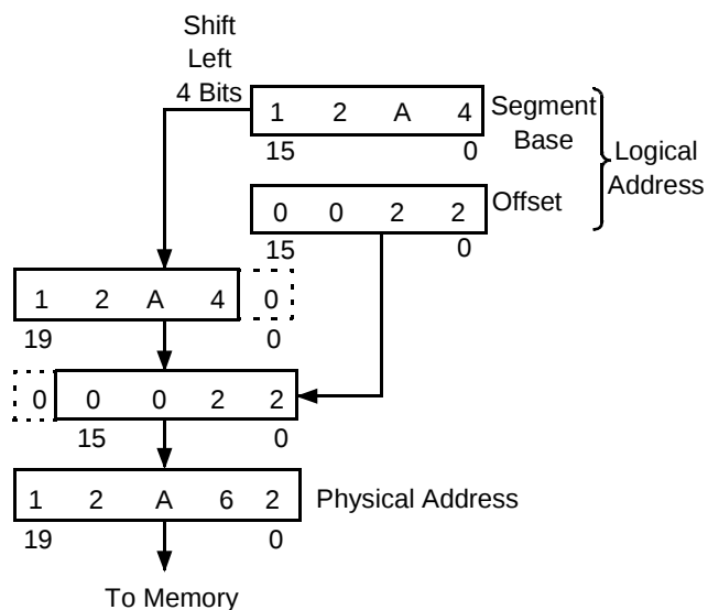
Figure 2. Two-Component Address
