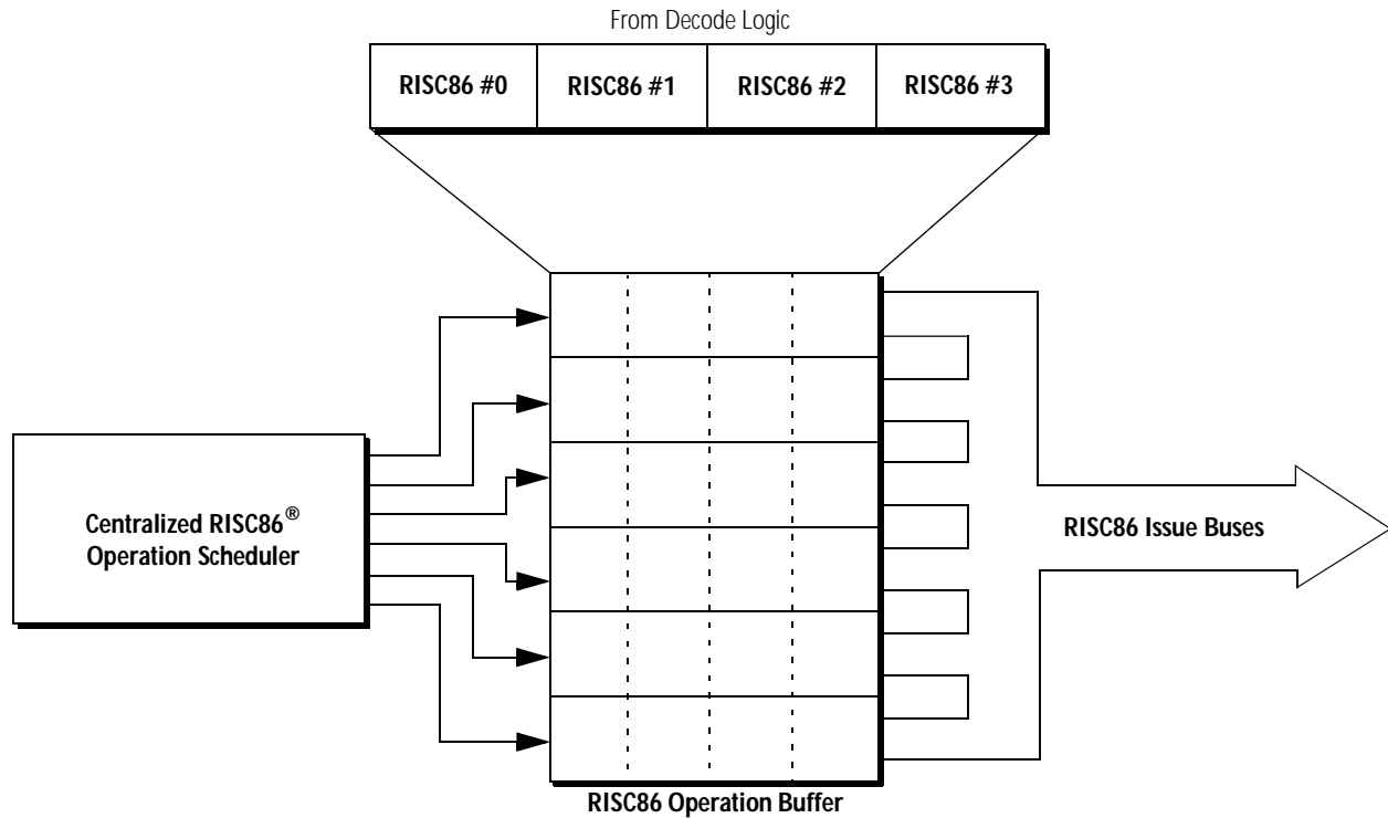
Figure 5. Mobile AMD-K6 ® -III+ Processor Scheduler
