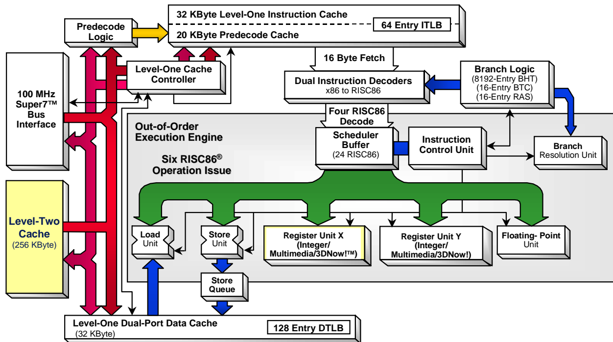
Figure 1. Mobile AMD-K6®-III+ Processor Block Diagram
