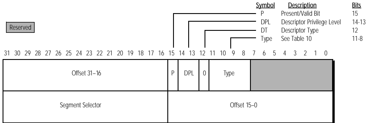
Figure 53. Gate Descriptor
