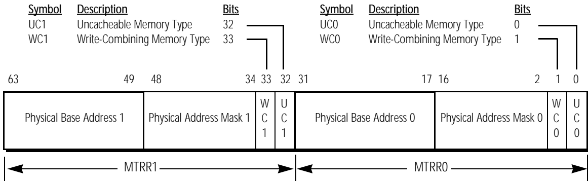
Figure 87. UC/WC Cacheability Control Register (UWCCR)—MSR C000_0085h
