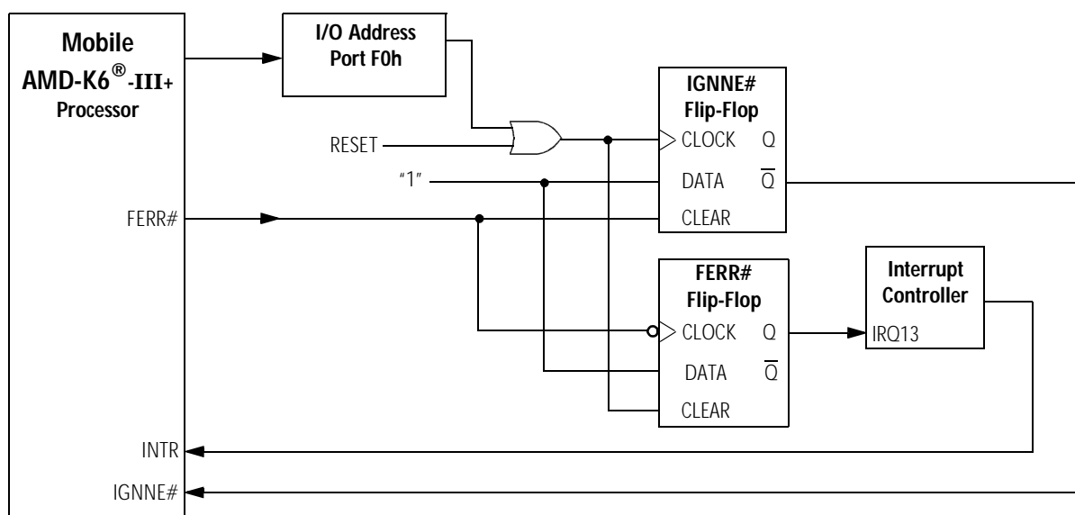
Figure 88. External Logic for Supporting Floating-Point Exceptions
