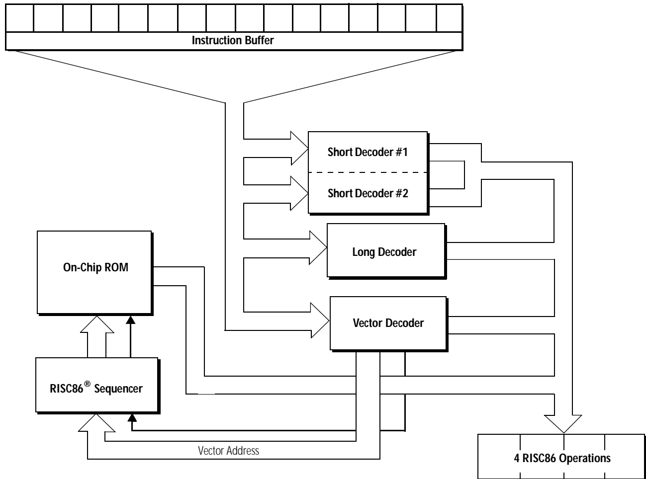
Figure 4. Mobile AMD-K6®-III+ Processor Decode Logic
