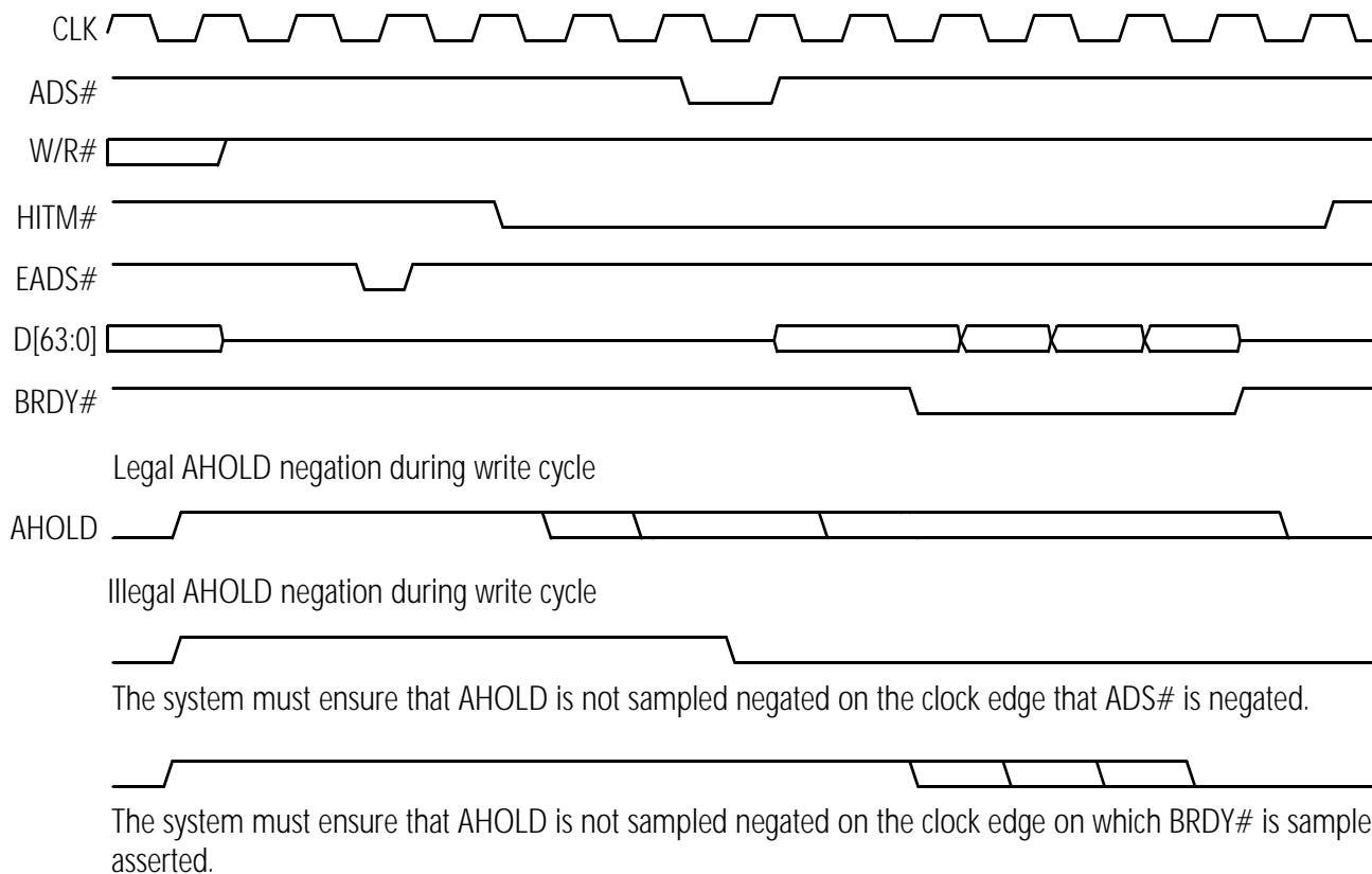
Figure 72. AHOLD Restriction
