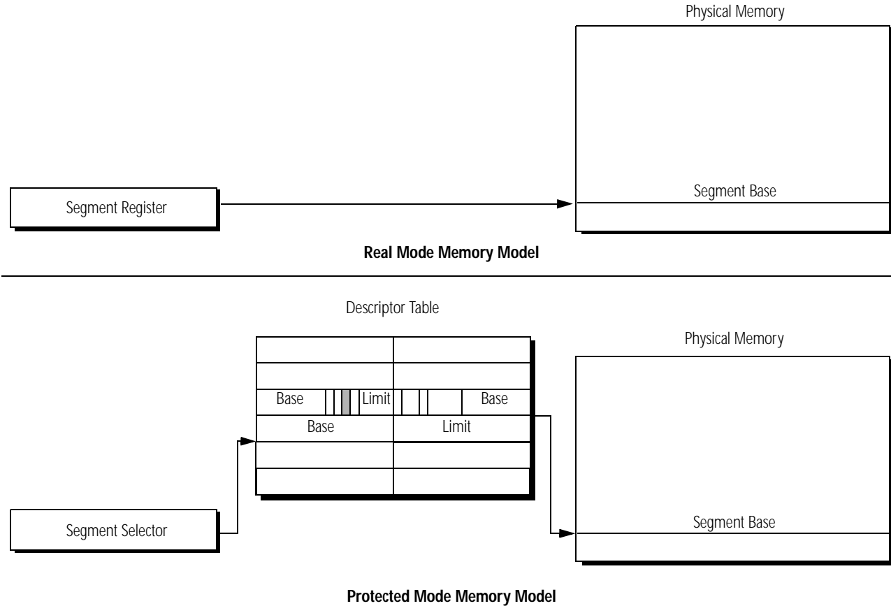
Figure 10. Segment Usage
