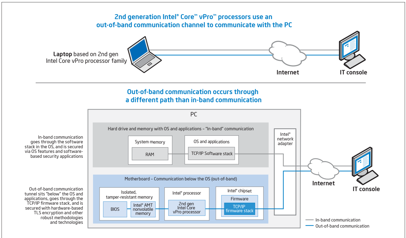
Figure 1. Out-of-band communication. Secure communication channel runs “under” or outside the OS. This channel is available regardless of the health of the operating system or the power state of the PC, even if the PC’s hard drive is removed.
