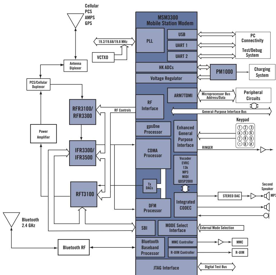
MSM3300 Device Functional Block Diagram
