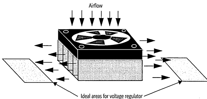
Figure 97. Airflow for a Heatsink with Fan
