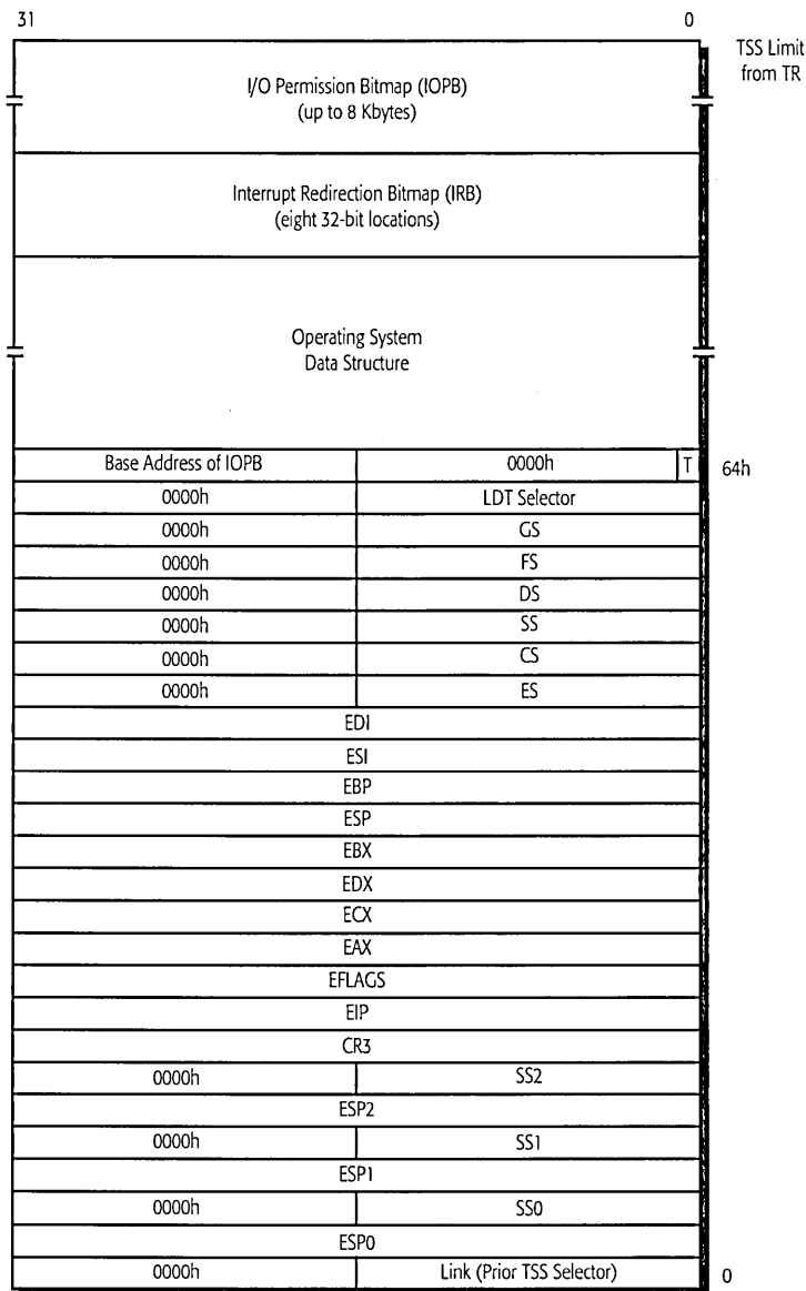
Figure 35. Task State Segment (TSS)
