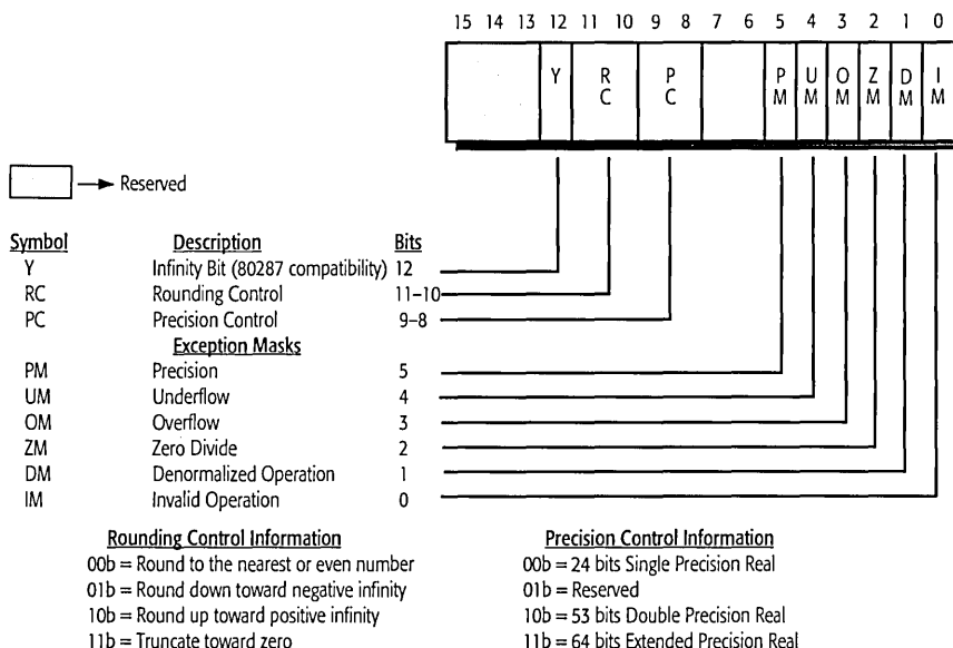
Figure 12. FPU Control Word Register
