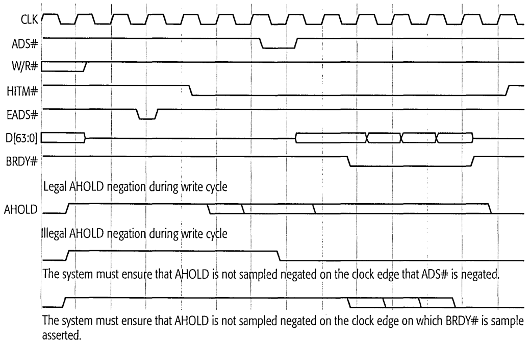
Figure 58. AHOLD Restriction
