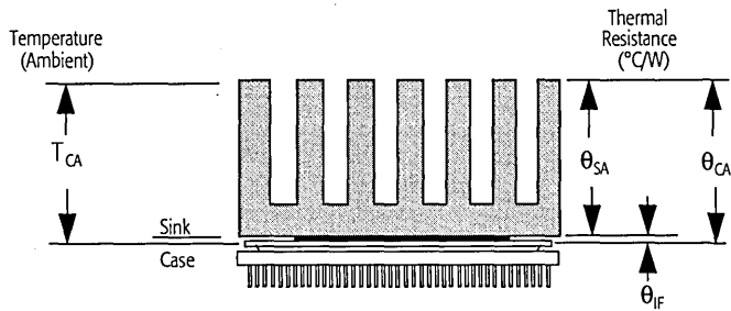
Figure 92. Thermal Model
