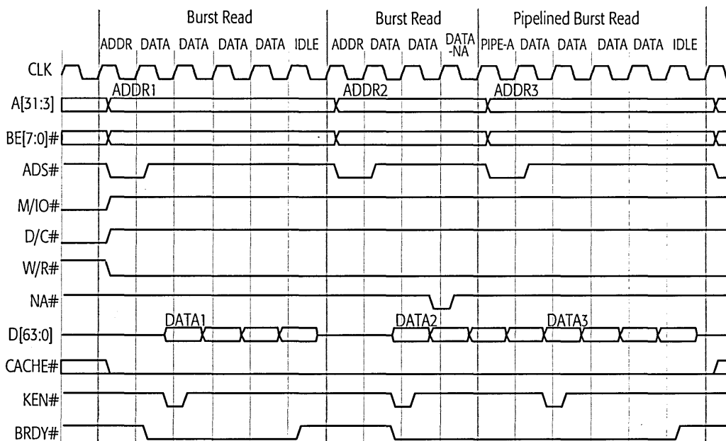
Figure 48. Burst Reads and Pipelined Burst Reads
