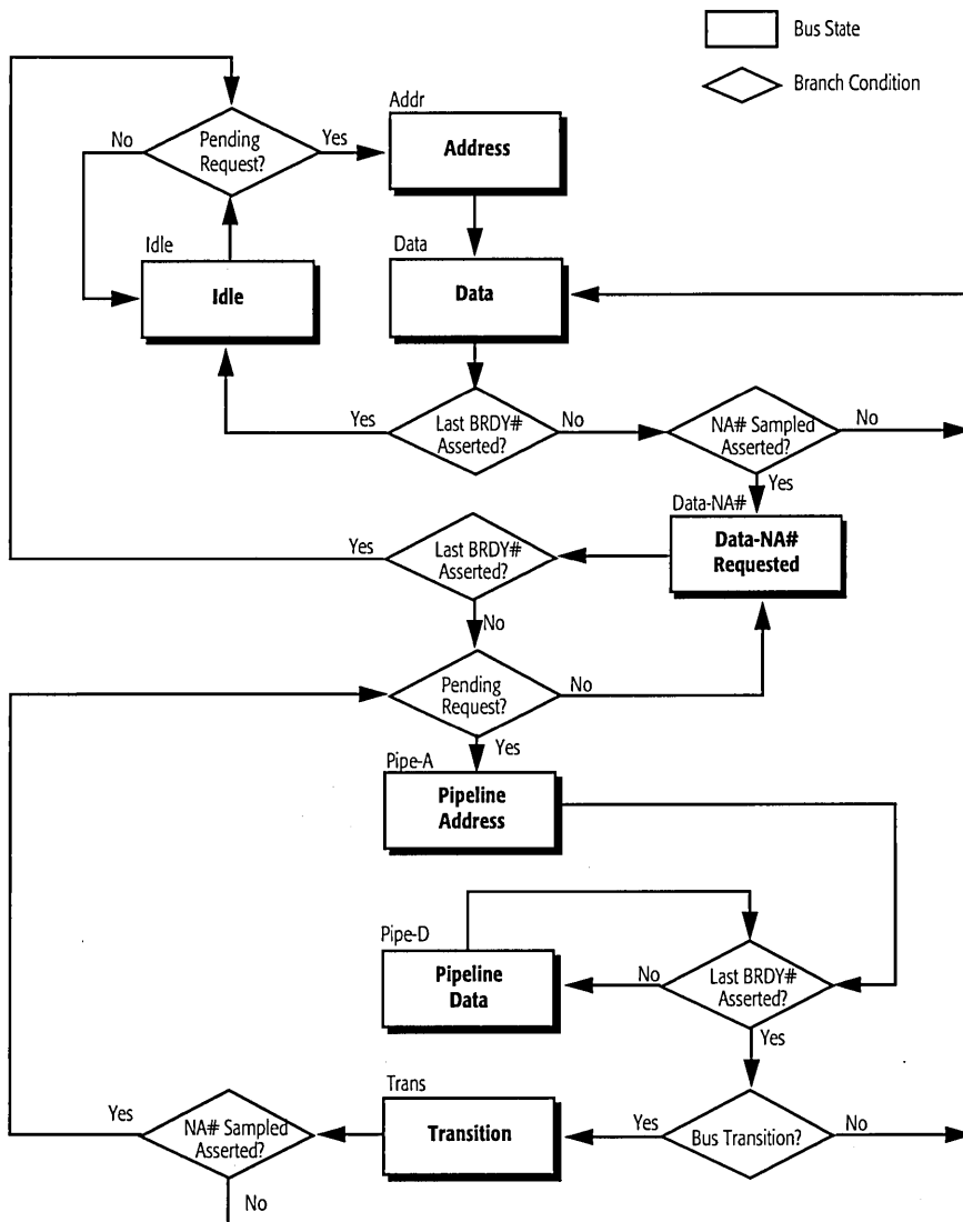
Figure 45. Bus State Machine Diagram
