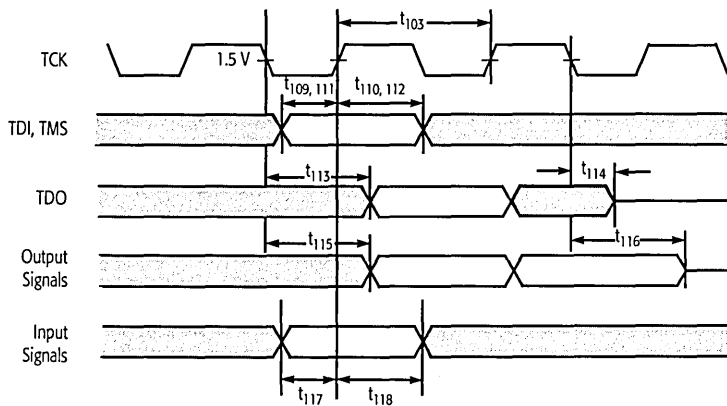
Figure 91. Test Signal Timing Diagram
