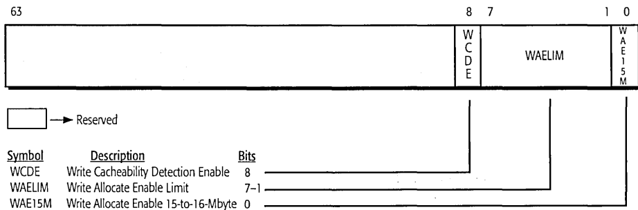
Figure 33. Write Handling Control Register (WHCR)
