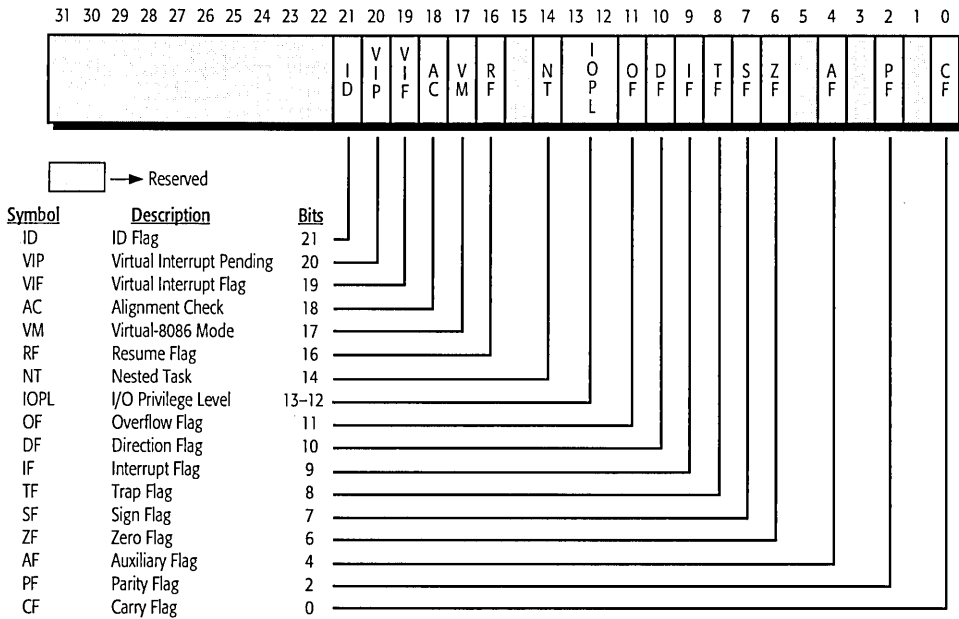
Figure 17. EFLAGS Registers
