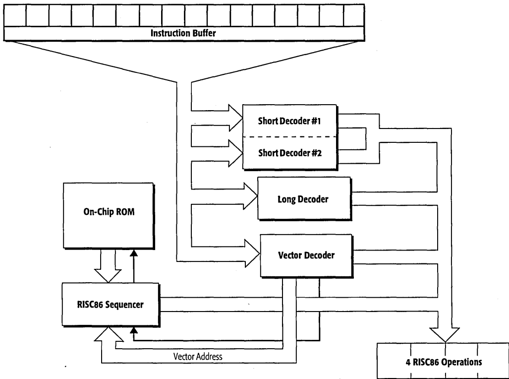
Figure 4. AMD-K6™ Processor Decode Logic
