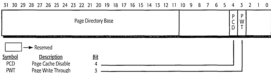
Figure 19. Control Register 3 (CR3)
