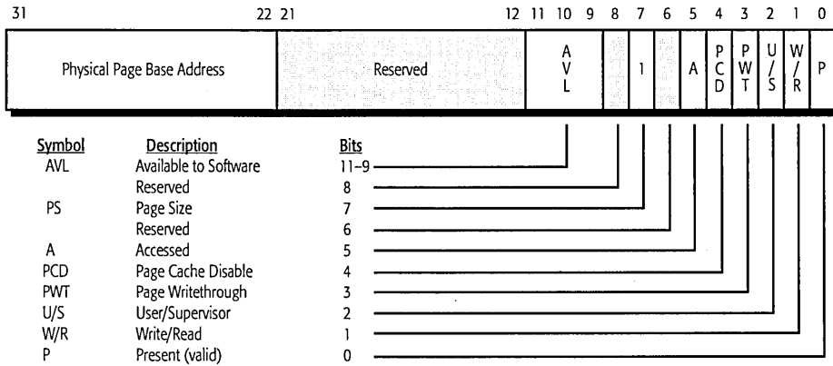
Figure 39. Page Directory Entry 4-Mbyte Page Table (PDE)
