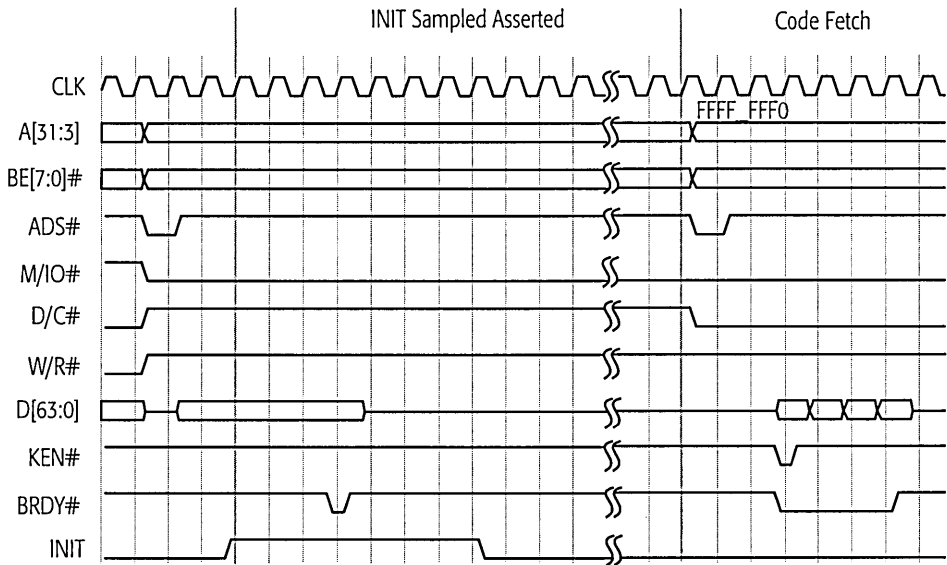
Figure 67. INIT-Initiated Transition from Protected Mode to Real Mode
