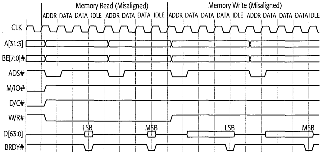
Figure 47. Misaligned Single-Transfer Memory Read and Write
