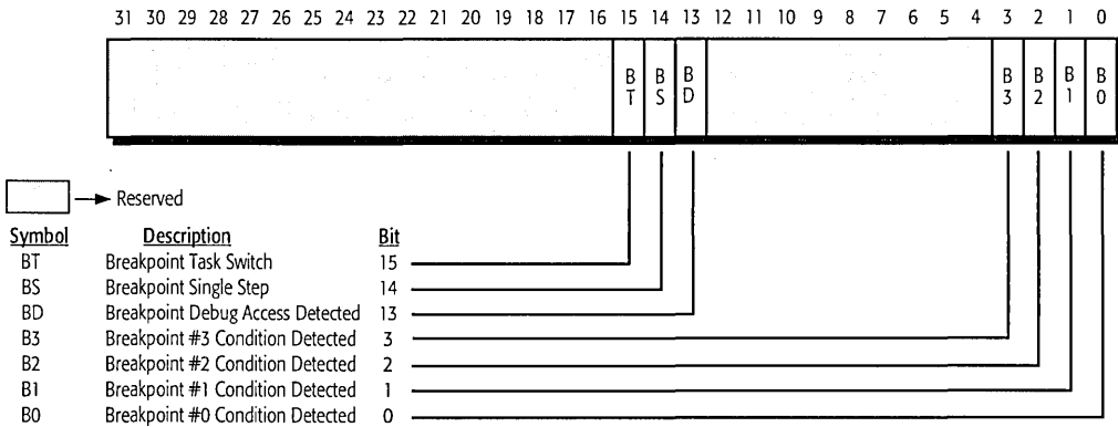
Figure 24. Debug Register DR6
