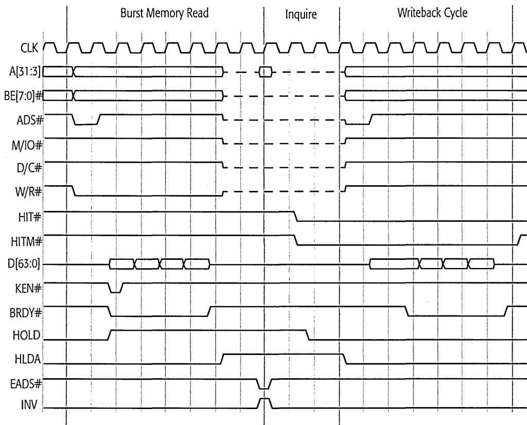
Figure 54. HOLD-Initiated Inquire Hit to Modified Line
