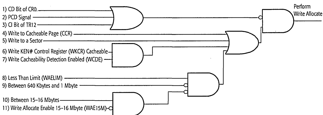
Figure 71. Write Allocate Logic Mechanisms and Conditions
