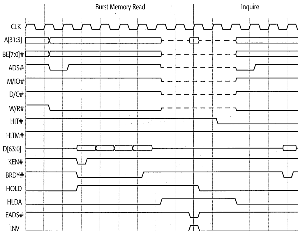
Figure 53. HOLD-Initiated Inquire Hit to Shared or Exclusive Line
