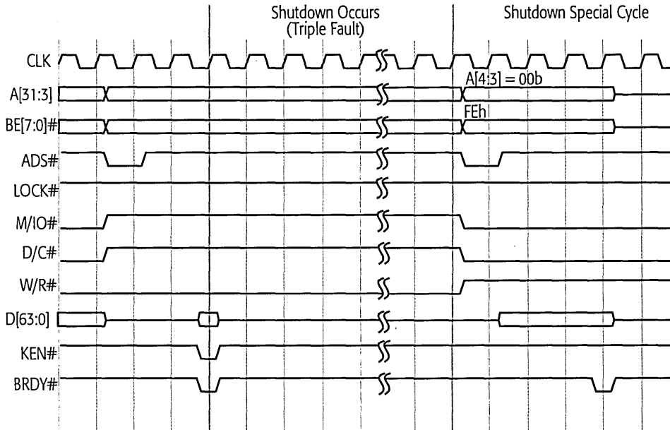
Figure 64. Shutdown Cycle
