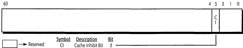
Figure 29. Test Register 12 (TR12)
