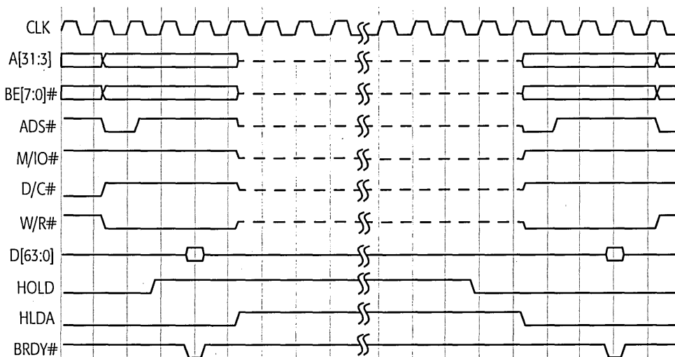
Figure 52. Basic HOLD/HLDA Operation
