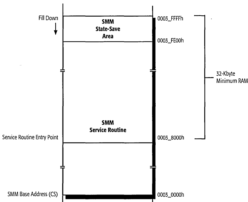
Figure 73. SMM Memory
