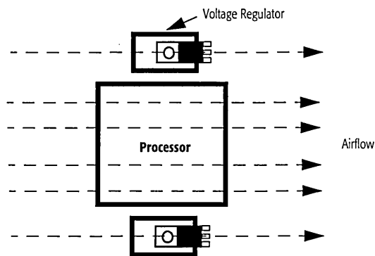
Figure 96. Voltage Regulator Placement
