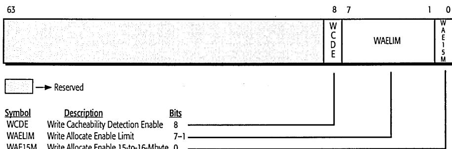
Figure 70. Write Handling Control Register (WHCR)
