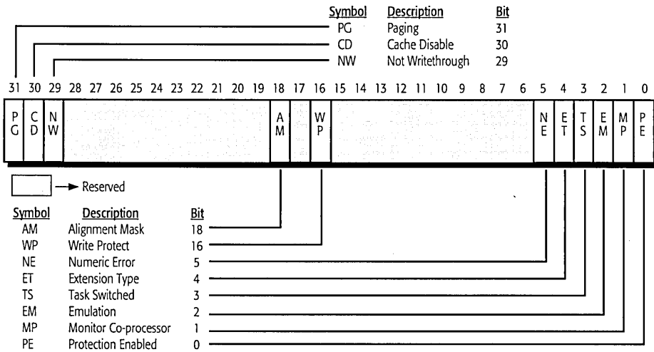
Figure 22. Control Register 0 (CR0)
