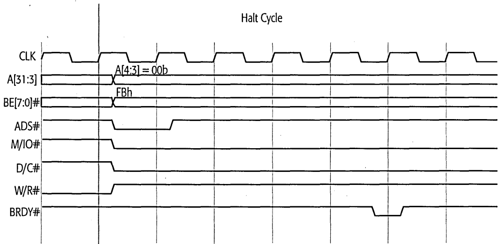
Figure 63. Basic Special Bus Cycle (Halt Cycle)
