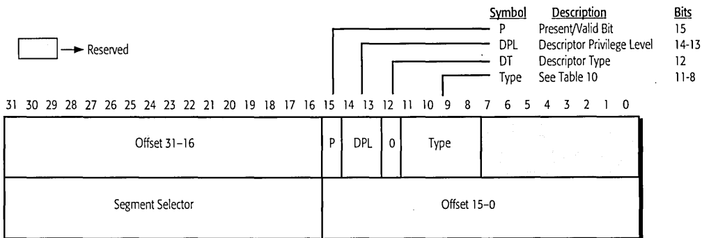
Figure 43. Gate Descriptor
