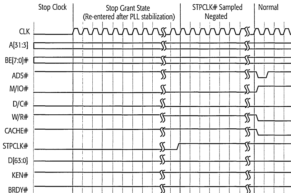
Figure 66. Stop Grant and Stop Clock Modes, Part 2
