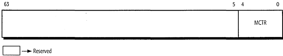
Figure 28. Machine-Check Type Register (MCTR)
