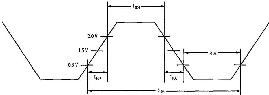
Figure 89. TCK Waveform
