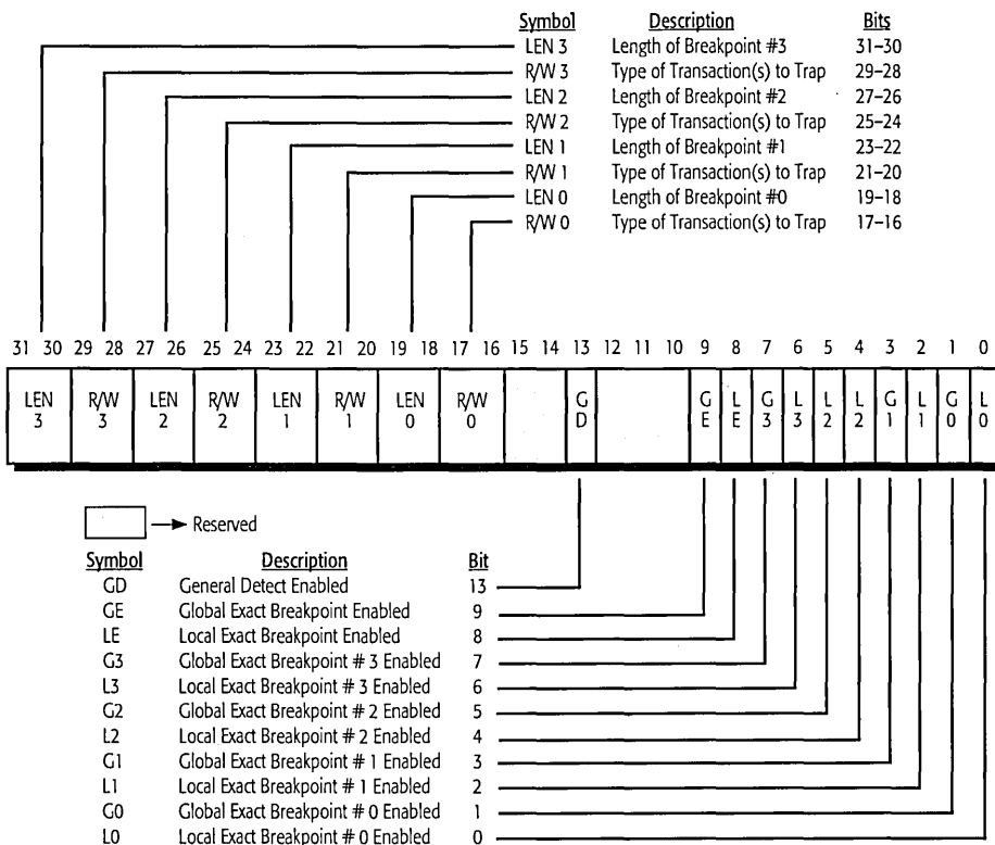
Figure 23. Debug Register DR7
