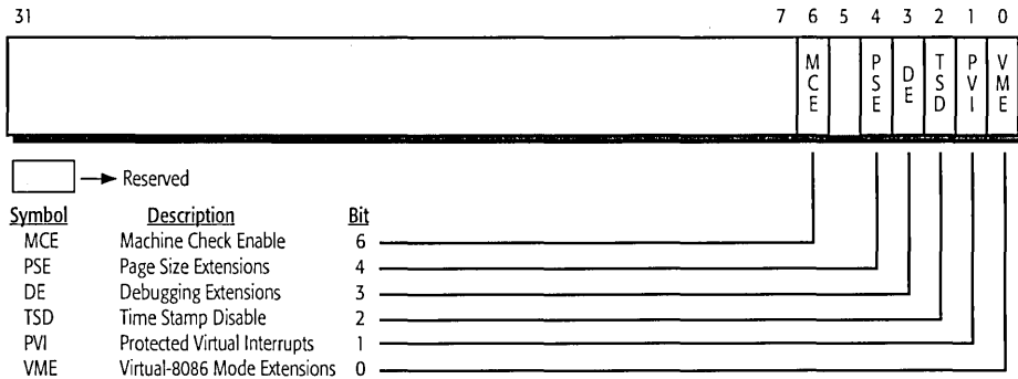
Figure 18. Control Register 4 (CR4)
