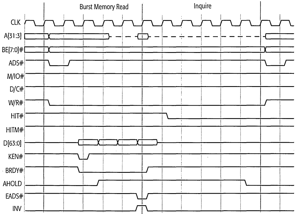
Figure 56. AHOLD-Initiated Inquire Hit to Share or Exclusive Line
