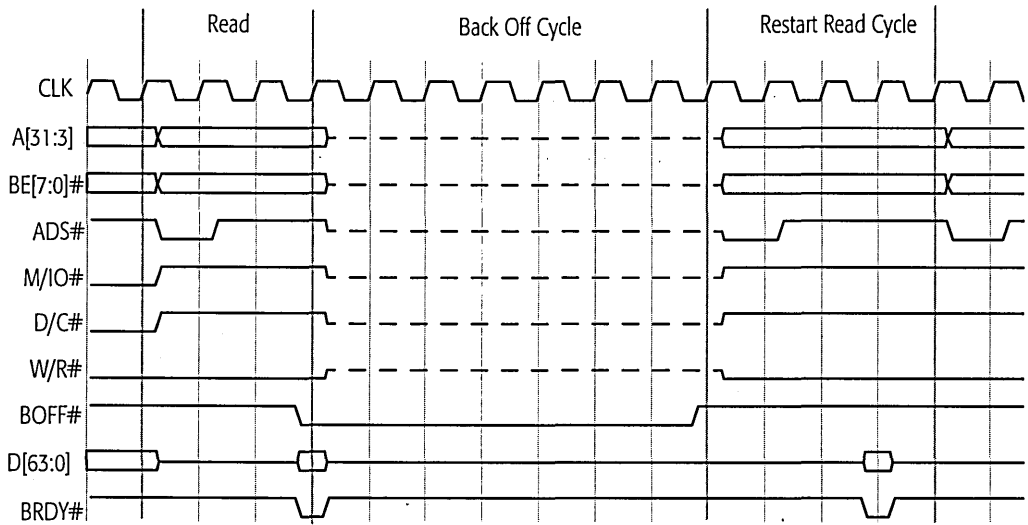
Figure 59. BOFF# Timing
