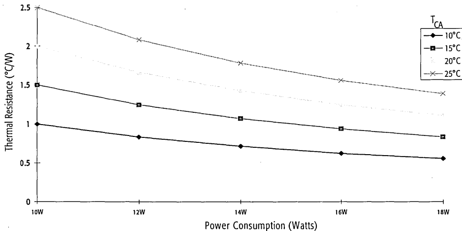
Figure 93. Power Consumption vs. Thermal Resistance
