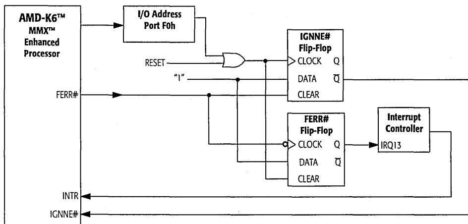
Figure 72. External Logic for Supporting Floating-Point Exceptions
