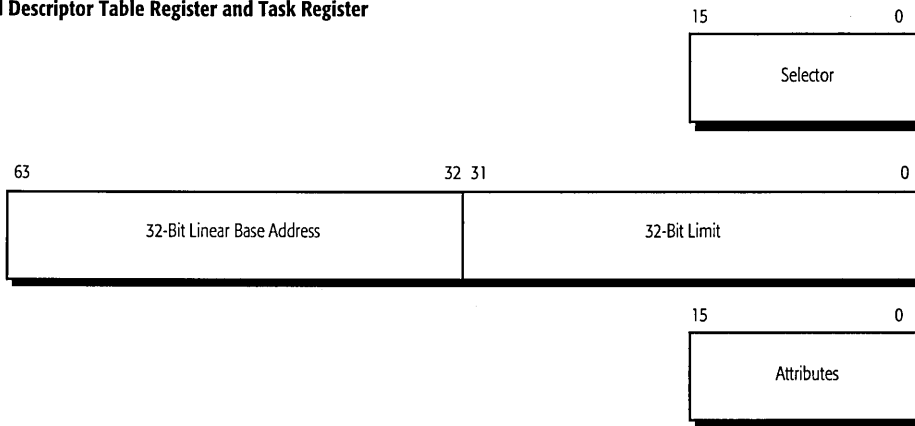
Figure 34. Memory Management Registers
