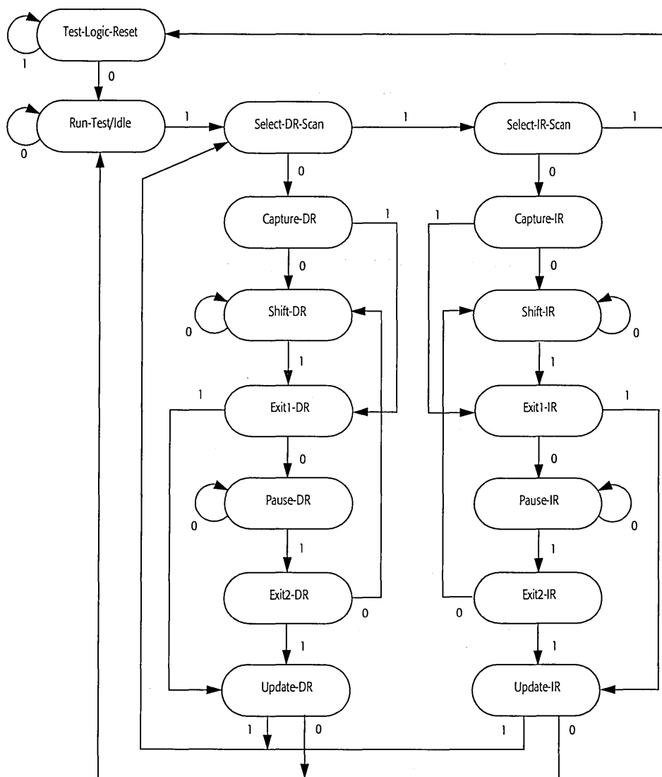
Figure 74. TAP State Diagram
