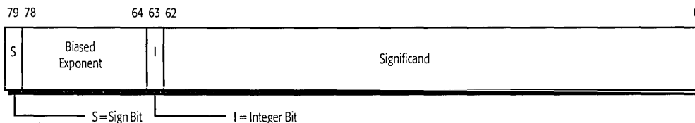
Figure 15. Precision Real Data Registers
