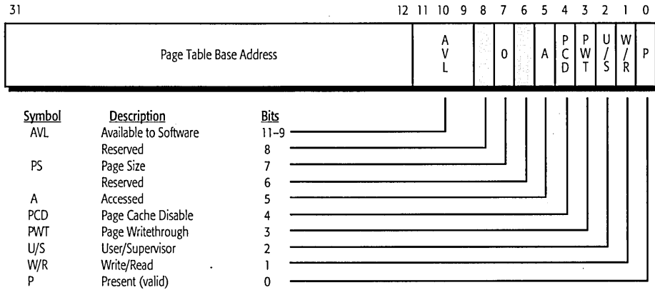
Figure 38. Page Directory Entry 4-Kbyte Page Table (PDE)
