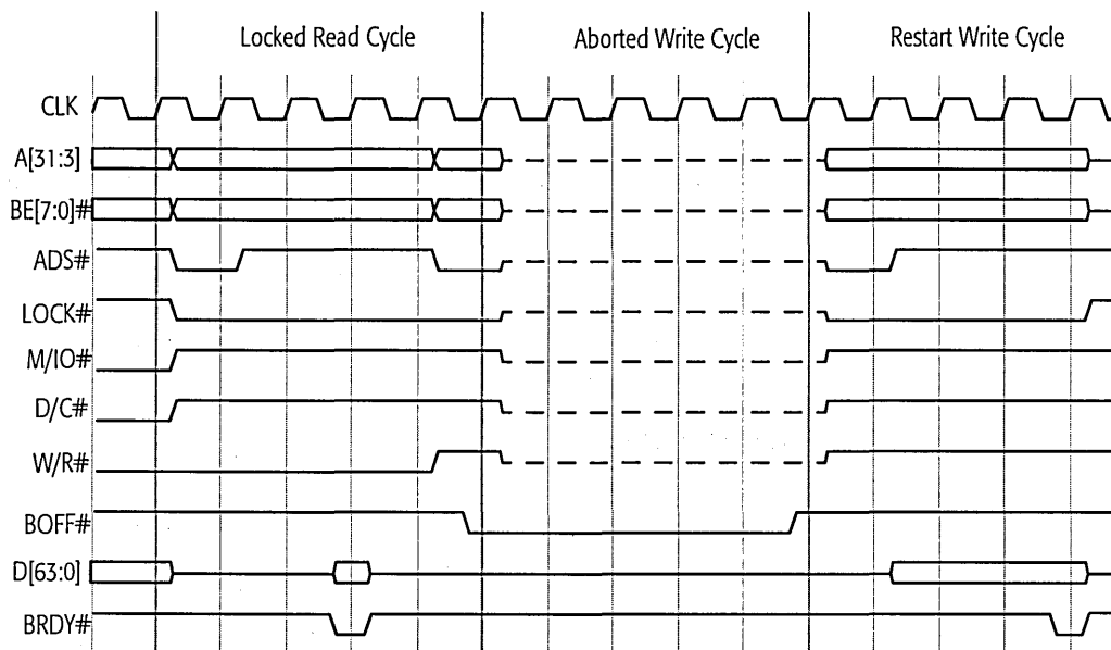
Figure 61. Locked Operation with BOFF\# Intervention
