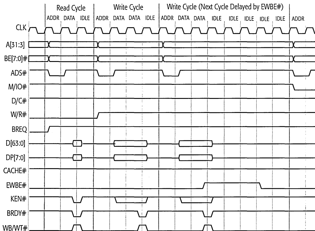
Figure 46. Non-Pipelined Single-Transfer Memory Read/Write and Write Delayed by EWBE#
