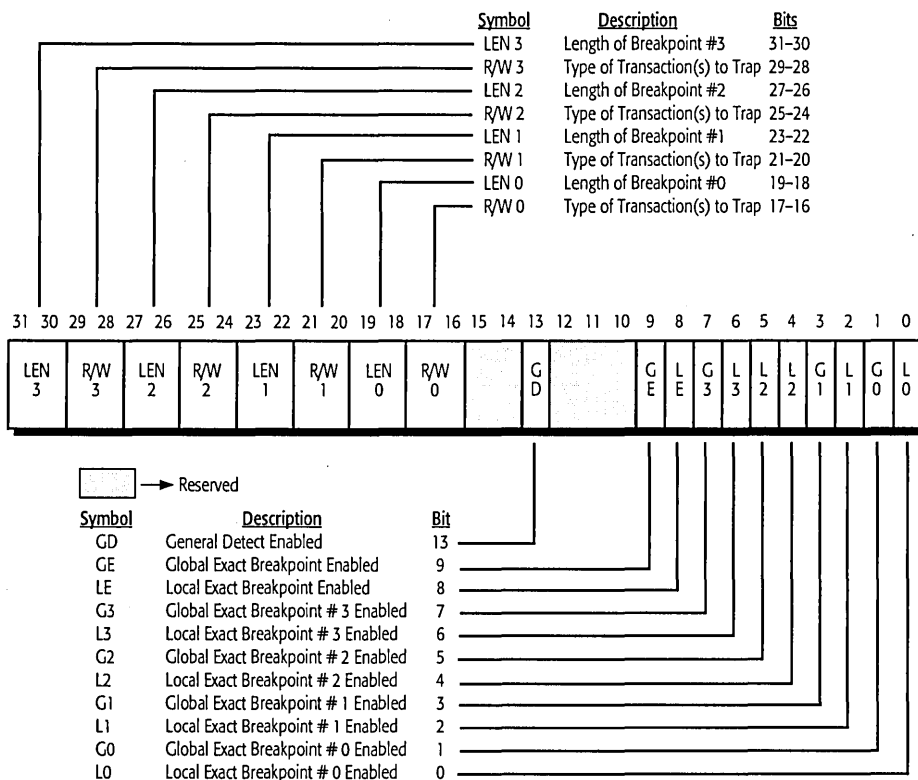
Figure 75. Debug Register DR7
