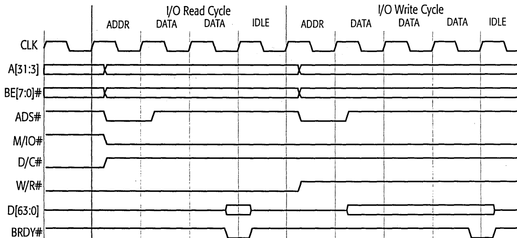
Figure 50. Basic I/O Read and Write
