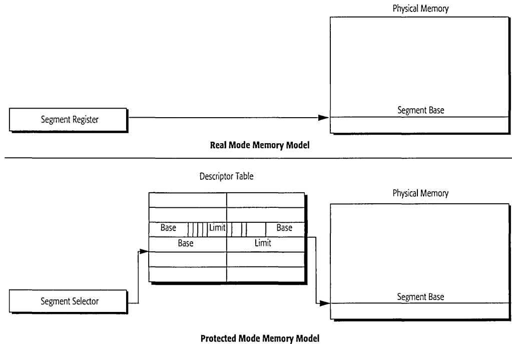
Figure 9. Segment Usage
