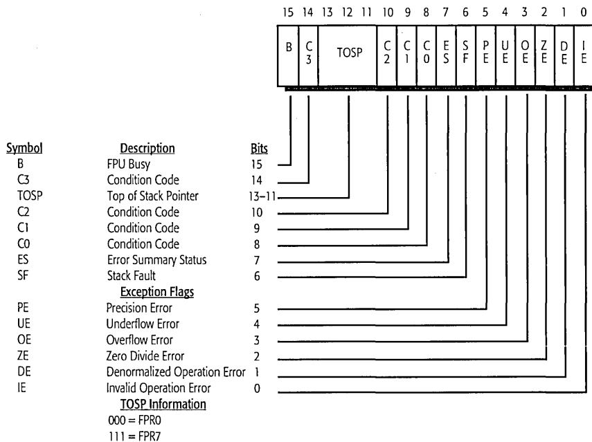
Figure 11. FPU Status Word Register
