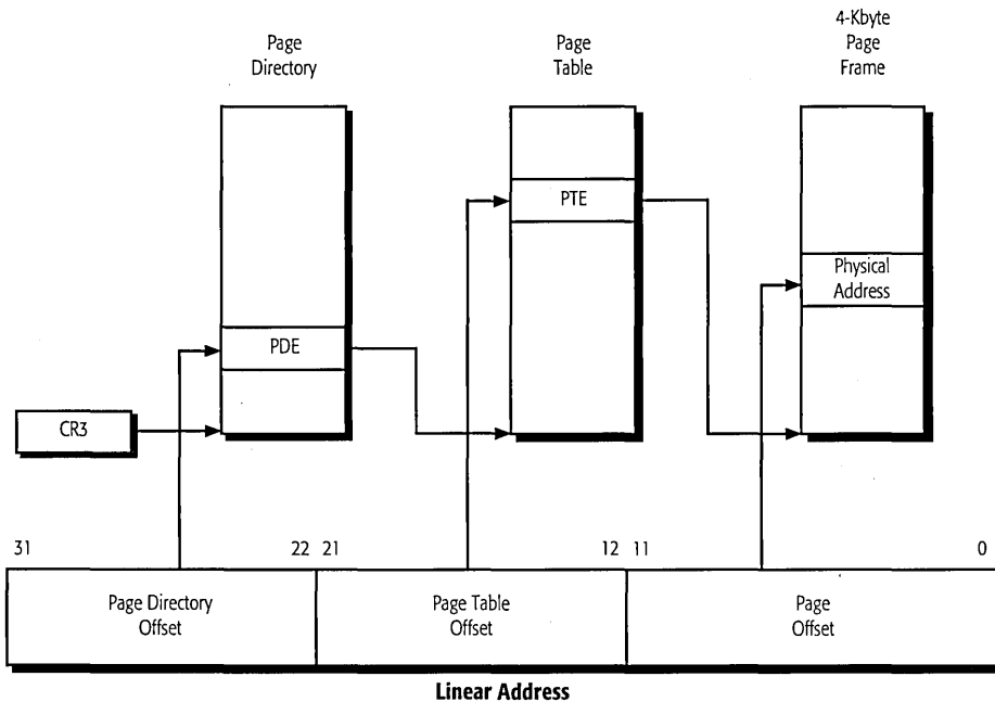
Figure 36. 4-Kbyte Paging Mechanism
