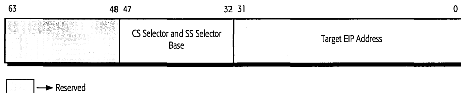
Figure 32. SYSCALL Target Address Register (STAR)
