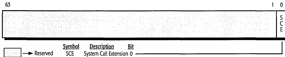
Figure 31. Extended Feature Enable Register (EFER)
