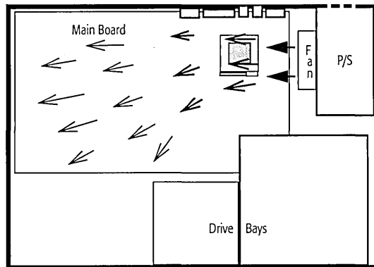
Figure 99. Airflow Path in an ATX Form-Factor System
