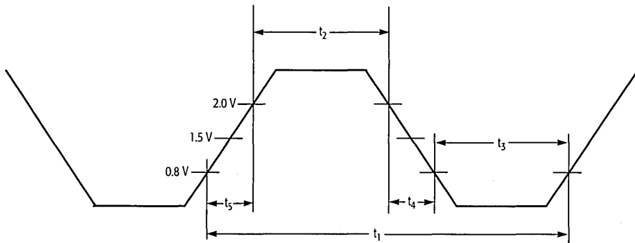
Figure 83. CLK Waveform
