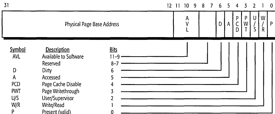
Figure 40. Page Table Entry (PTE)
