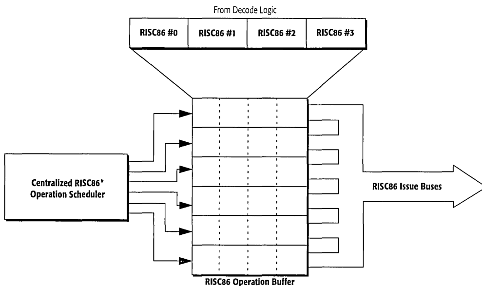
Figure 5. AMD-K6™ Processor Scheduler
