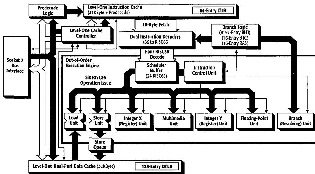
Figure 1. AMD-K6™ MMX™ Enhanced Processor Block Diagram
