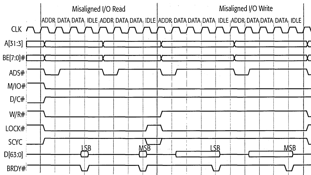
Figure 51. Misaligned I/O Transfer
