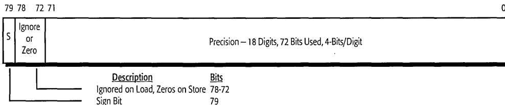
Figure 14. Packed Decimal Data Register
