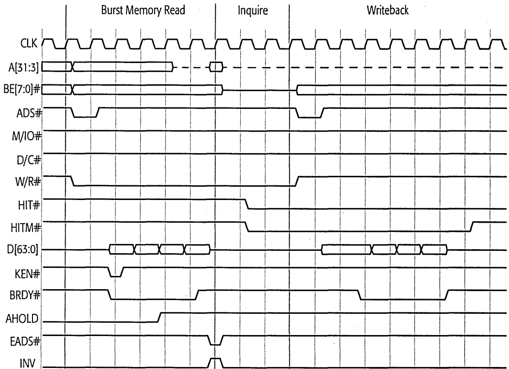
Figure 57. AHOLD-Initiated Inquire Hit to Modified Line
