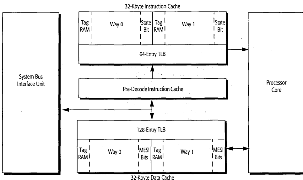
Figure 68. Cache Organization
