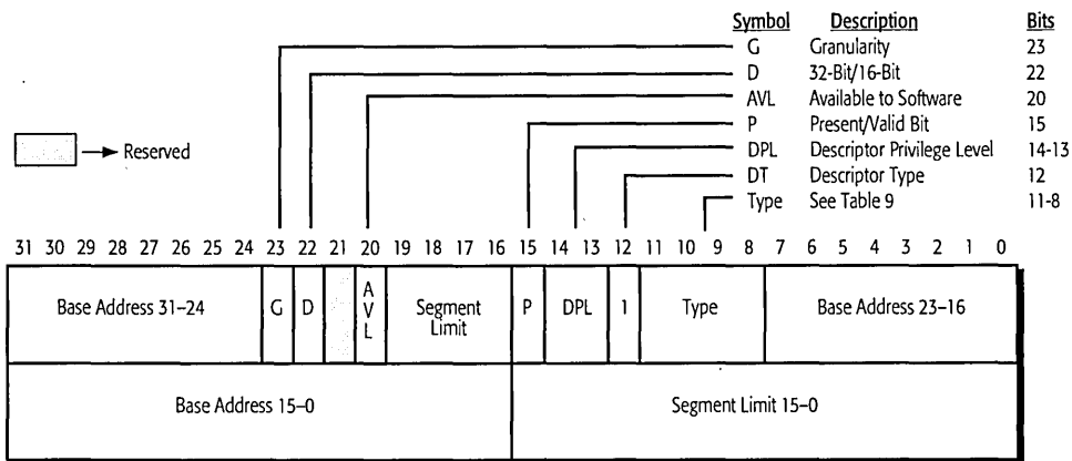
Figure 41. Application Segment Descriptor
