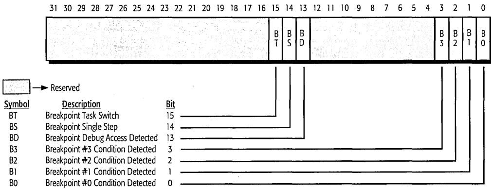
Figure 76. Debug Register DR6
