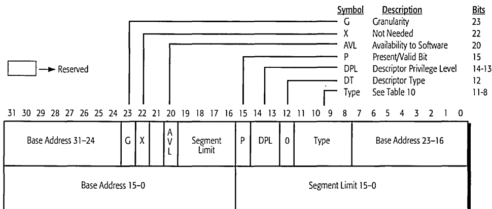
Figure 42. System Segment Descriptor
