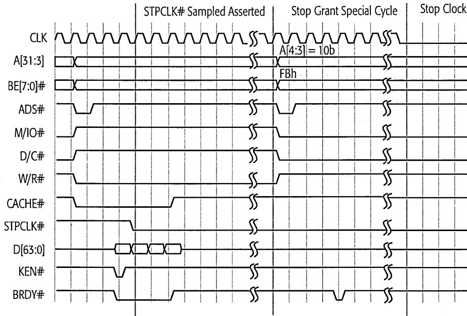
Figure 65. Stop Grant and Stop Clock Modes, Part 1
