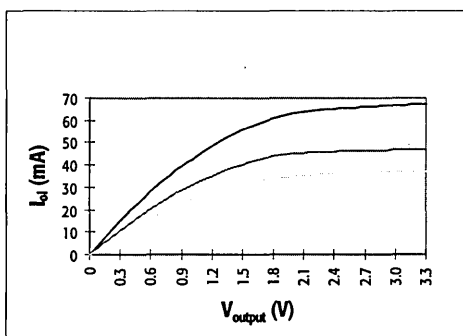
Figure 81. K6STD Pulldown V/I Curves
