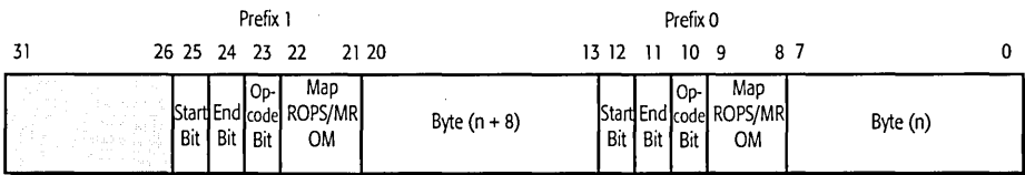
Figure 10. Test Formats: Icache Instructions for the AMD-K5™ Processor Model 1 and Greater
