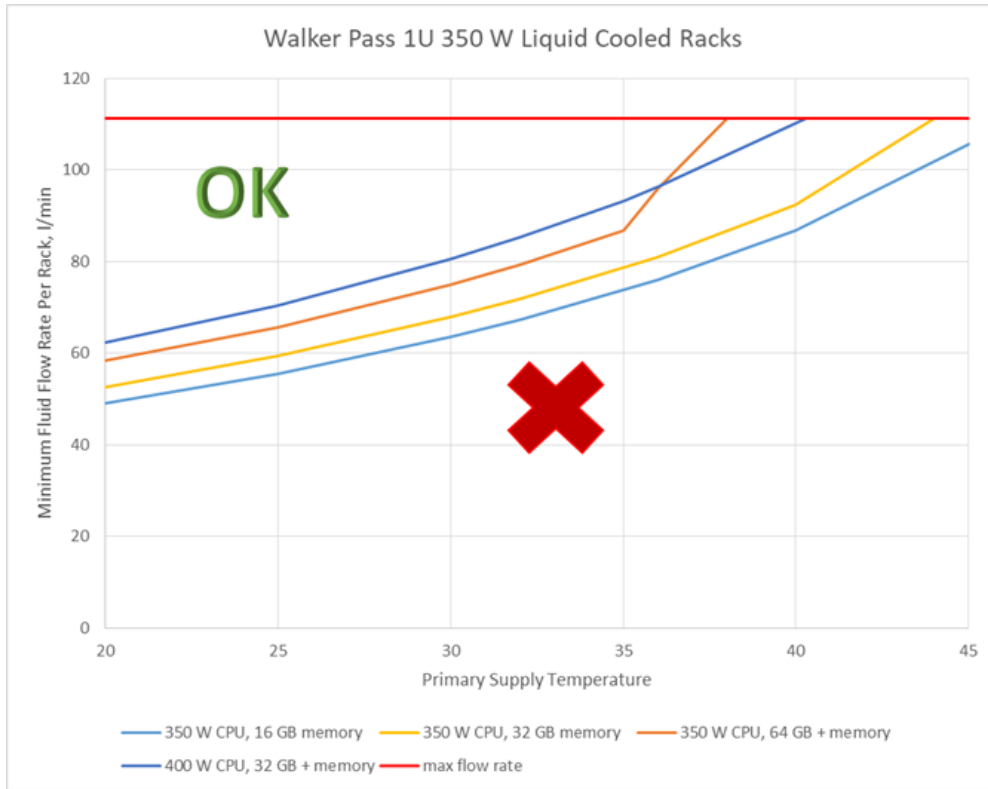
Figure 3. Fluid flow requirement per system at each inlet
