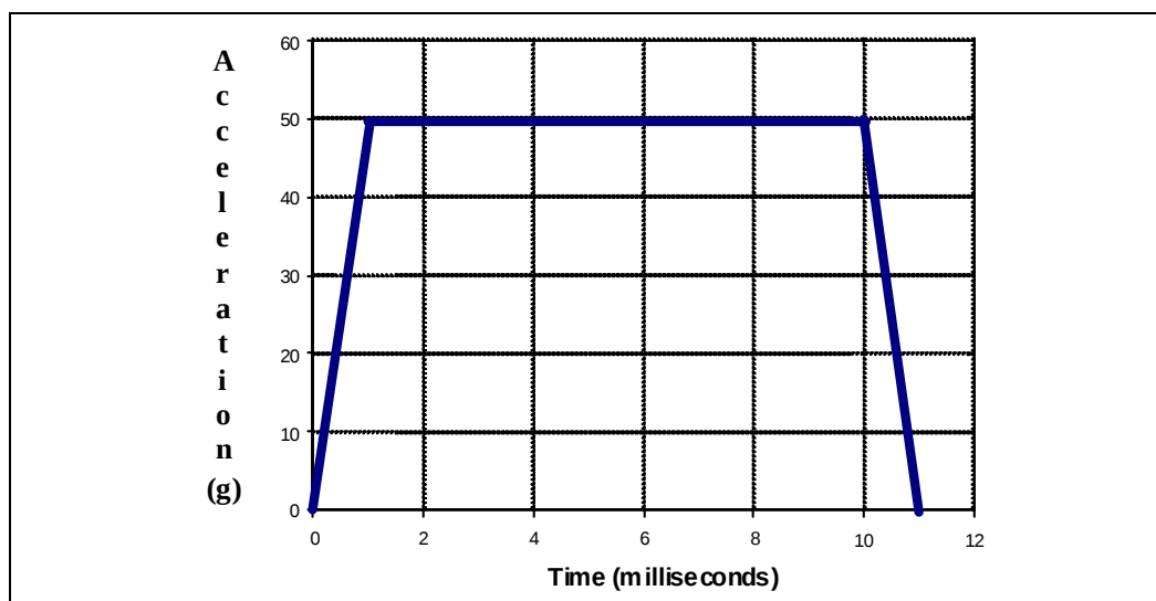
Figure 10. Shock Acceleration Curve
