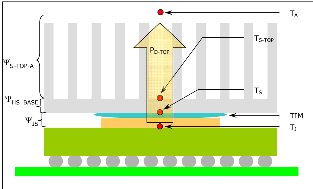
Figure 4. Processor Thermal Characterization Parameter Relationships
