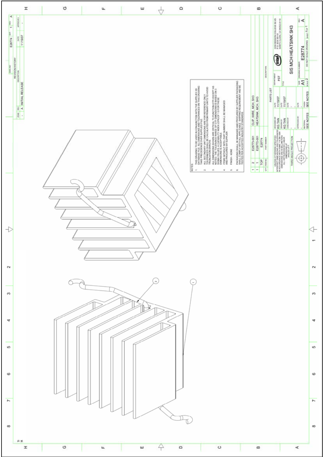
Figure 19. SiS671 GMCH Reference Thermal Solution for Intel® Atom™ Processor 200 Series / SiS Chipset Platform (E28774-001)
