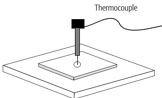
Figure 23. Measuring Case Temperature
