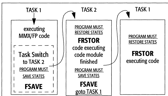
FIGURE 2-1. Cooperative Task Switching
