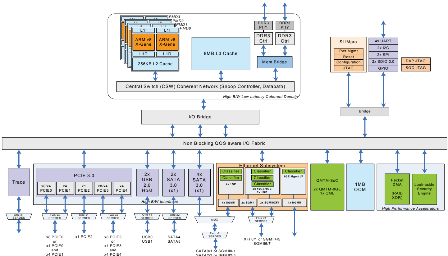
X-Gen 1 Block Diagram
