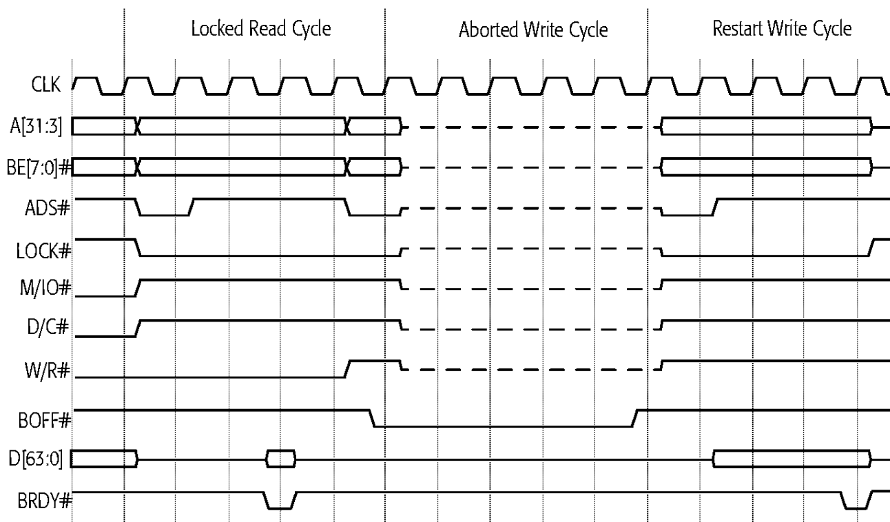
Figure 60. Locked Operation with BOFF# Intervention
