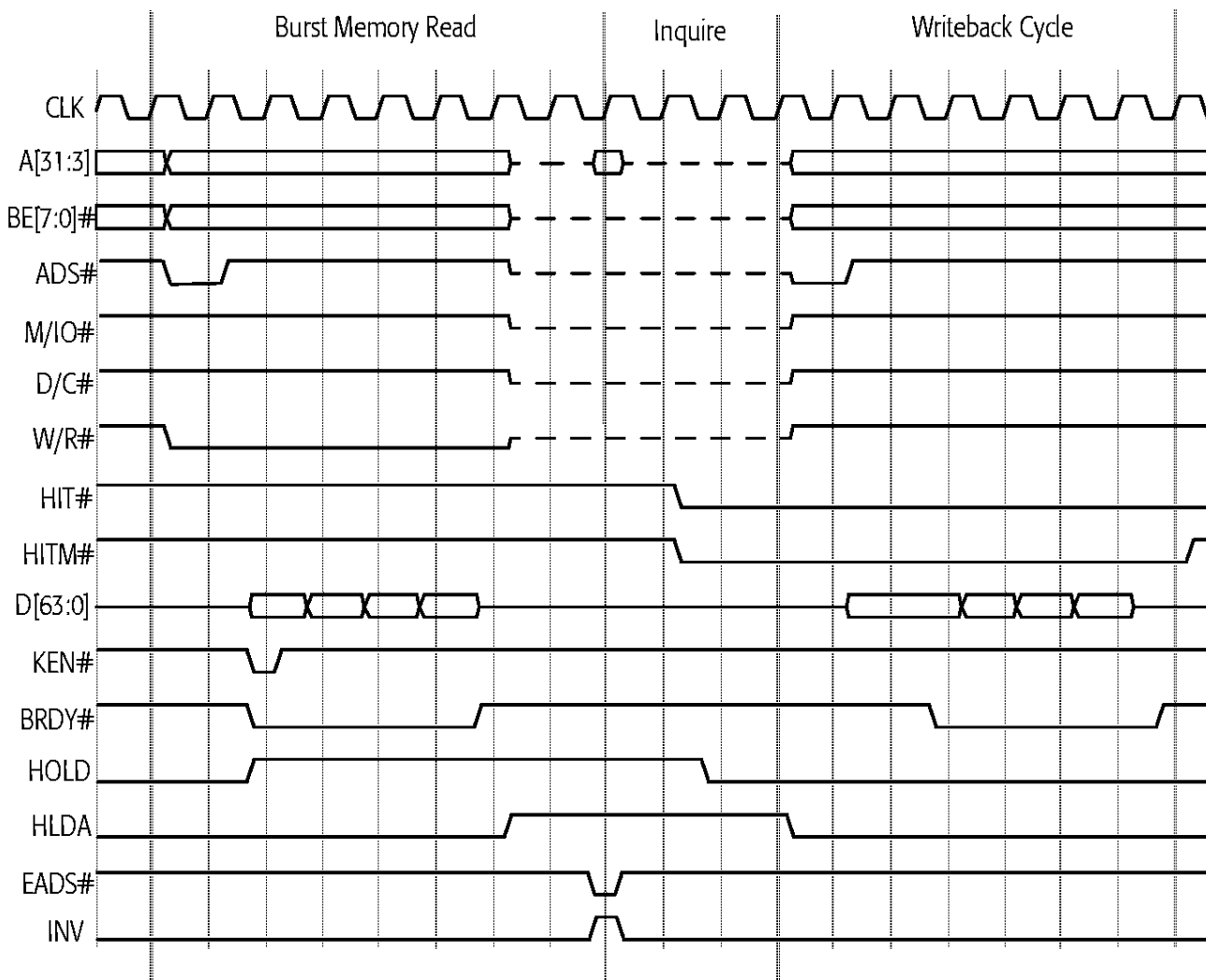
Figure 53. HOLD-Initiated Inquire Hit to Modified Line
