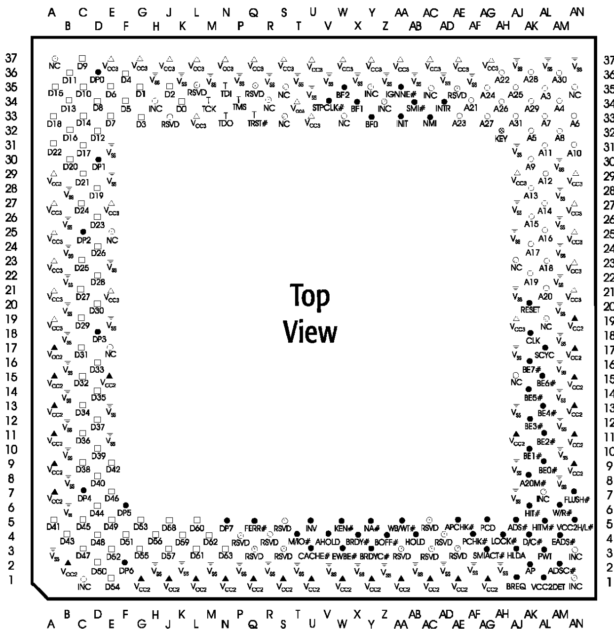
Figure 104. AMD-K6® Processor Model 7 Top-Side View
