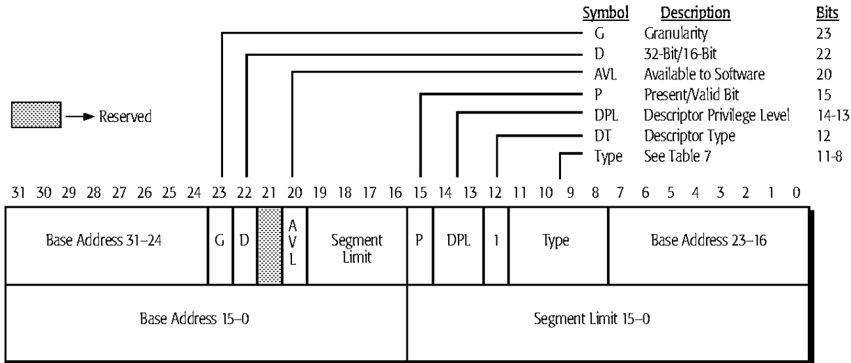
Figure 40. Application Segment Descriptor
