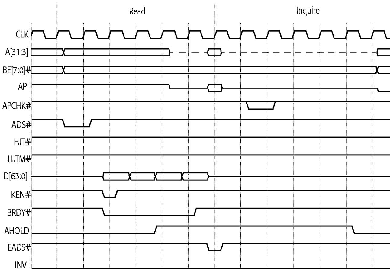
Figure 54. AHOLD-Initiated Inquire Miss
