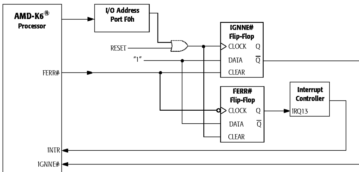
Figure 71. External Logic for Supporting Floating-Point Exceptions
