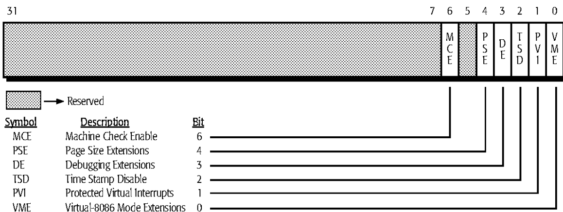
Figure 19. Control Register 4 (CR4)
